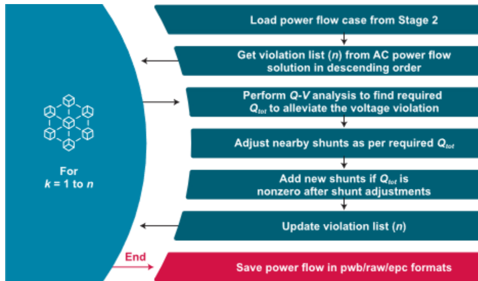
Figure D.11. Reactive power planning to improve voltage profiles.
