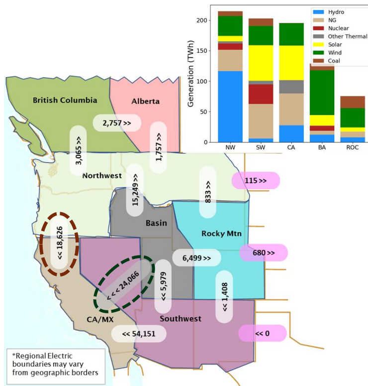
Figure 26. Net interregional energy transfers (GWh) for the Base case (top) and High RE case (bottom).
