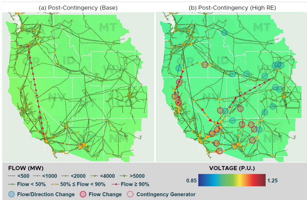
Figure 40. Comparison of voltage heatmaps and flows post-contingency between the (a) Base and (b) High RE cases for the same contingency of 2600 MW of generation loss.
